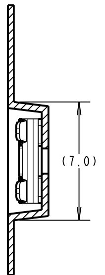
SECTION X-X
