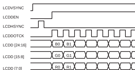
Figure 44-8. TFT Timing (First Line Expanded View)
