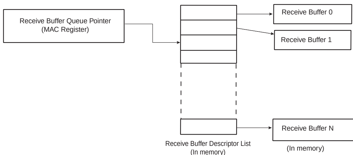
Figure 37-2. Receive Buffer List
