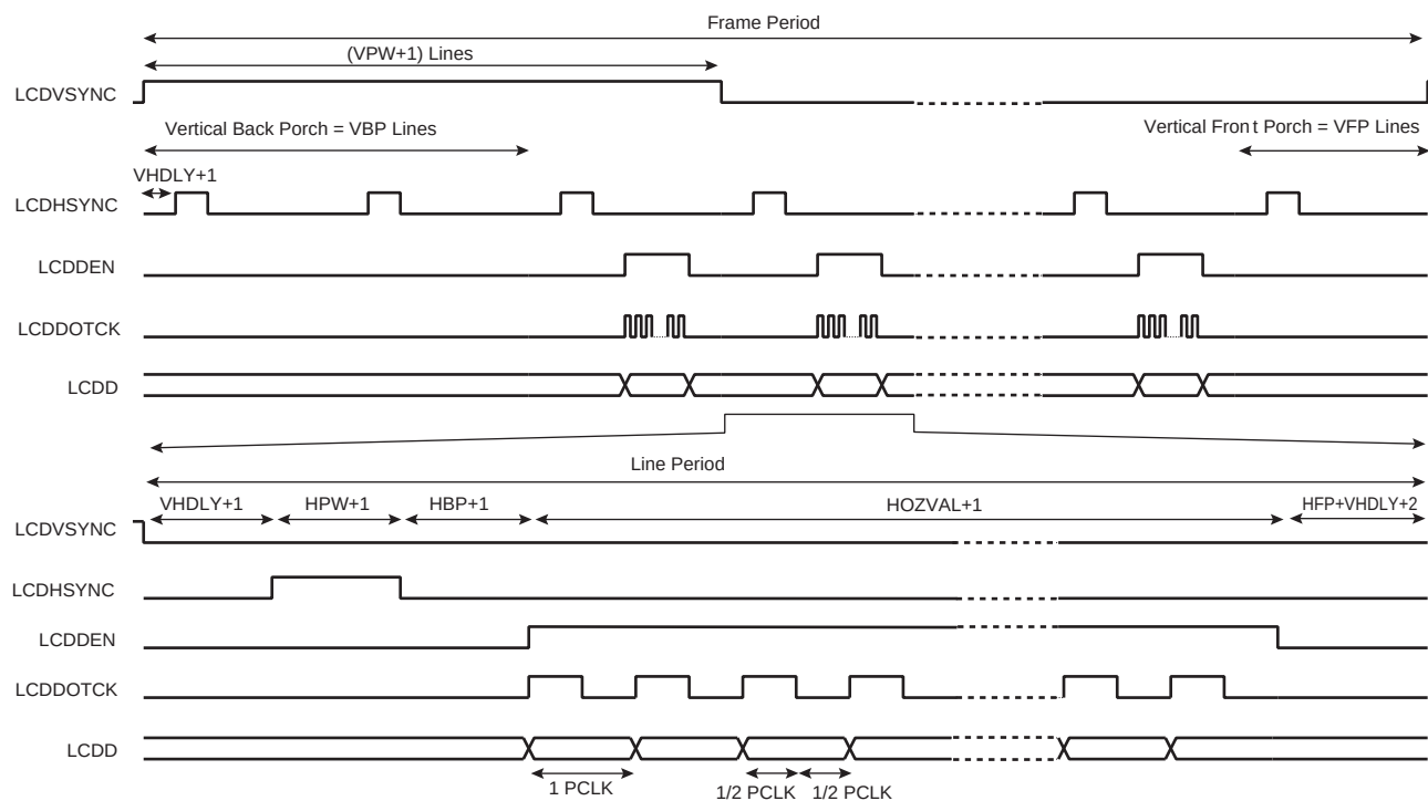
Figure 44-6. TFT Panel Timing, CLKMOD = 0, VPW = 2, VBP = 2, VFP = 1
