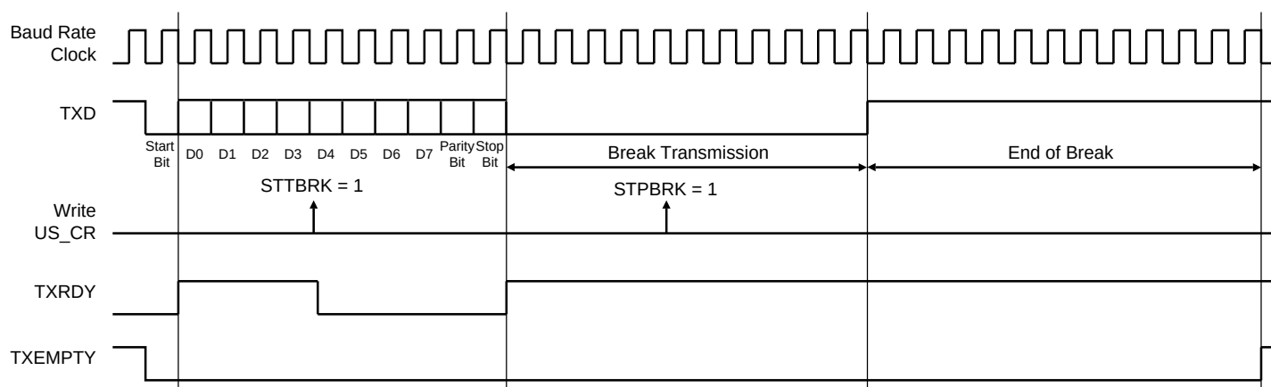
Figure 30-26. Break Transmission
