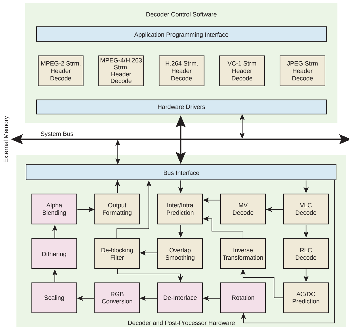
Figure 45-1. Block Diagram
