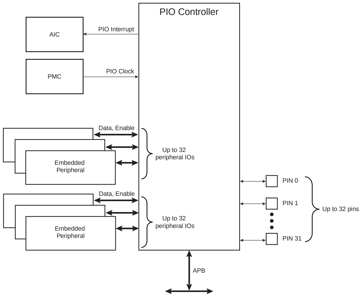
Figure 29-1. Block Diagram
