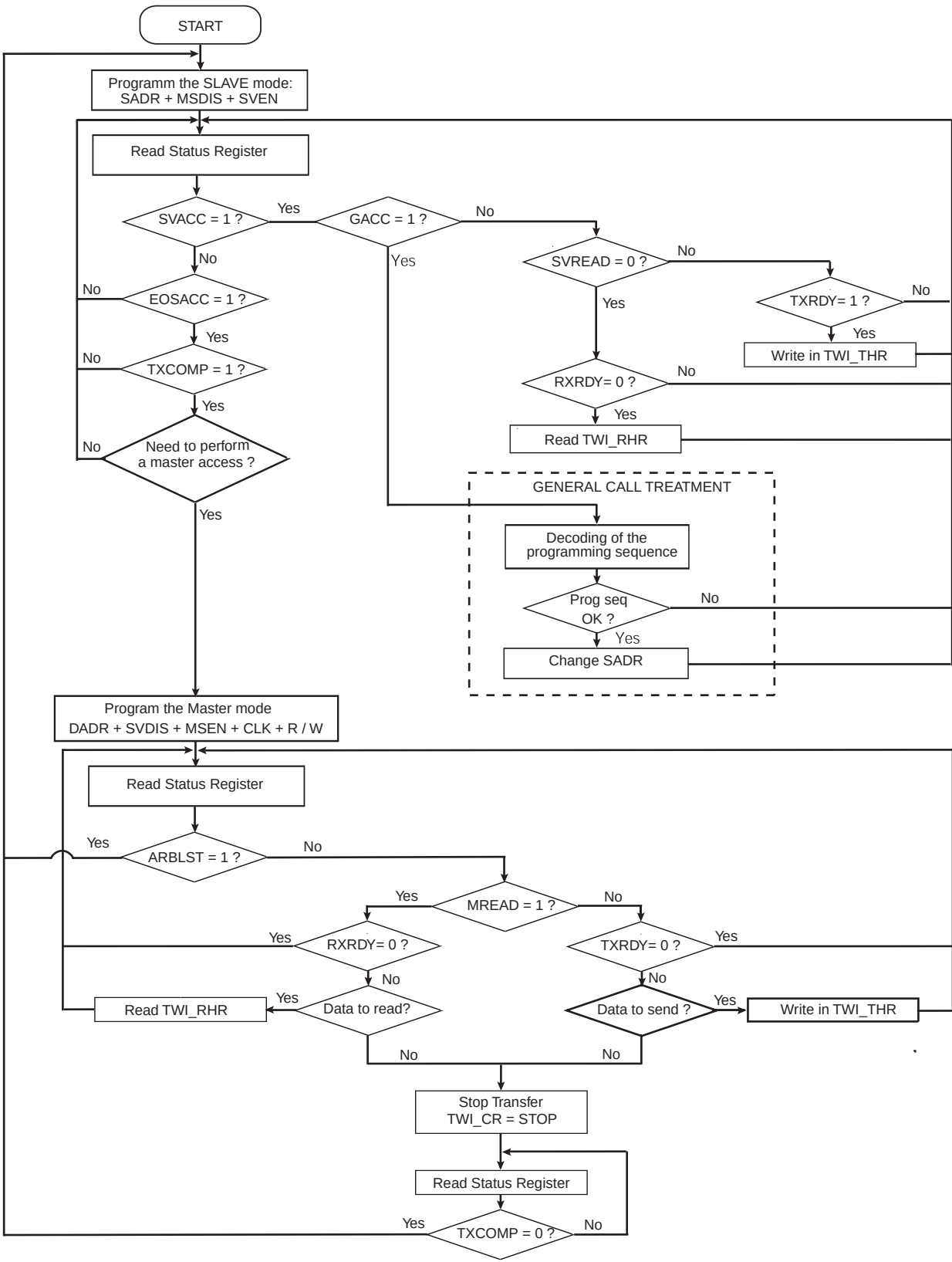
Figure 31-23. Multi-master Flowchart
